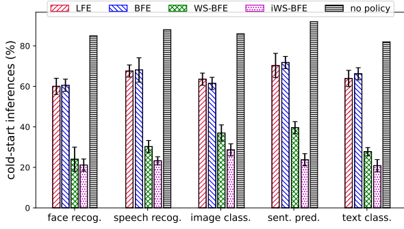
Fig. 9: The percentage of cold-start inferences using different NN model eviction policies versus no policy.
